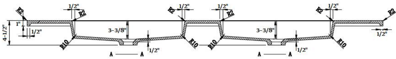
MODD 4922-1-107S DOUBLE BASINS
