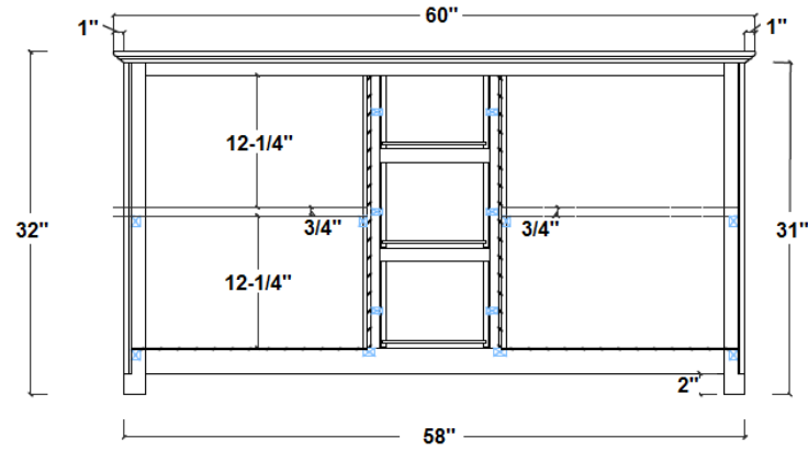
BACK/DERRIERE
