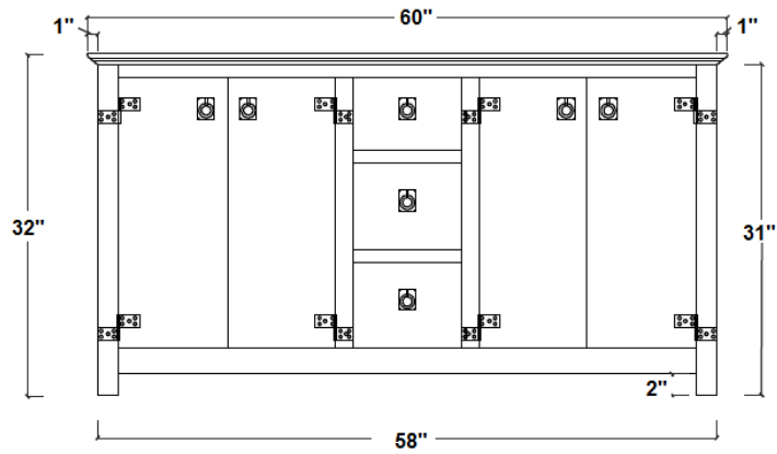
FRONT/DEVANT
