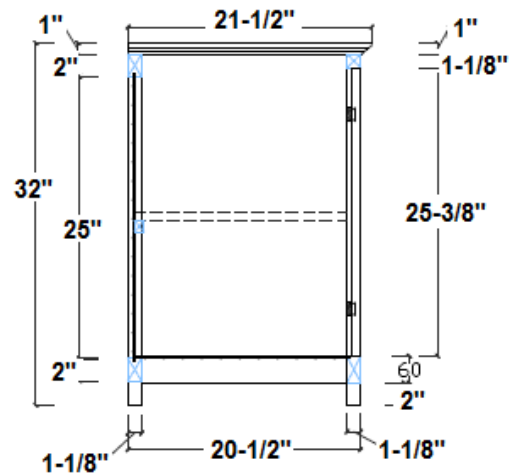
SIDE/COTE
