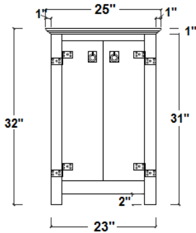
FRONT/DEVANT
